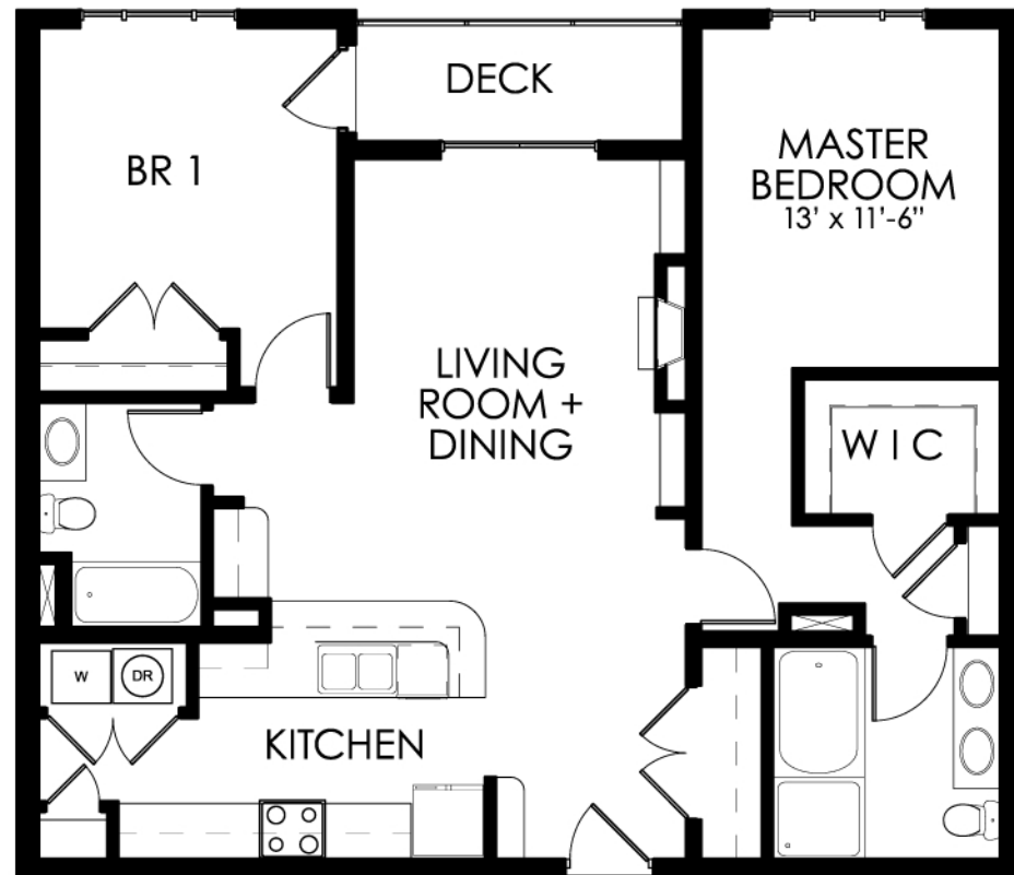
2 BR UNIT PLAN 900 SF
